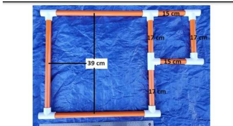
The designated area for the ADCP with the sediment area attached. The designated area is constructed from 1/2-inch PVC pipe.
